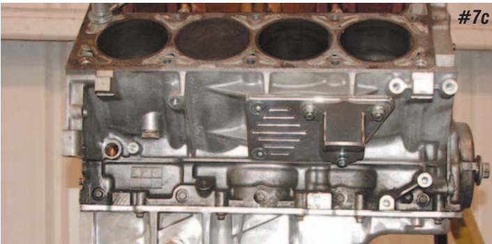
Photos #7a, #7b & #7c: We carry a modified GM cast aluminum oil pan P/N 18-228 that is designed to clear the steering component. This pan includes the oil pump pick up and pan gasket. For a more custom look, fully fabricated sheet metal oil pans are also available P/N 18-374 in steel or P/N 18-375 in aluminum. All three pans will work with the stock drag link or the CCI rack and pinion unit.
