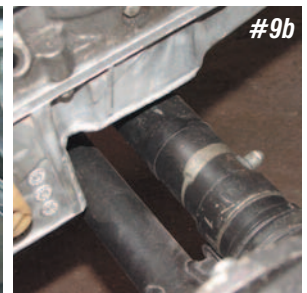
Photos #9a & #9b: You can see how much steering linkage clearance there is with the modified oil pan. The left photo shows the stock drag link and the right photo shows the rack and pinion.
