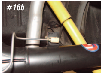
Photo #16a & 16b & 16c: The kit includes pre-bent brake lines that connect the calipers to the original brass junction block T on the rear end. The lines are bent to match up with the contour of the Ford rear and clip into the stock tabs on the rear end.
