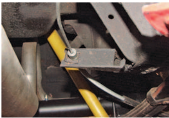
Photo #14: The cable should normally be routed under the tailpipes. Our project car has a custom exhaust system that would not allow that. With the cable connected to the linkage, adjust the linkage so that the rear emergency brakes are activated with the emergency brake handle pulled out half way.
