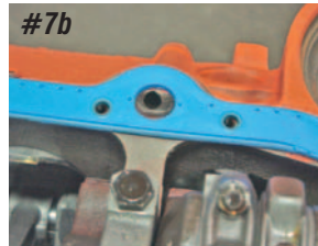
Photo #7a & 7b: The one-piece oil pan gasket will just about fall into place. All of the oil pan bolt holes and the dipstick hole will line up perfectly. Installation is a breeze even if the engine is in the car. When installing the silicone oil pan gasket, no gasket sealer is needed.
