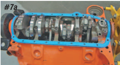
Photo #7a & 7b: The one-piece oil pan gasket will just about fall into place. All of the oil pan bolt holes and the dipstick hole will line up perfectly. Installation is a breeze even if the engine is in the car. When installing the silicone oil pan gasket, no gasket sealer is needed.
