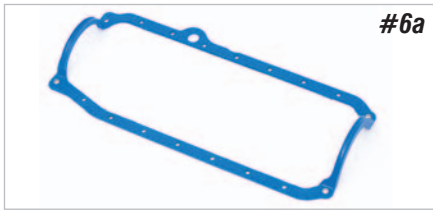
Photo #6a & 6b: Here is the answer to this long-time problem; a one-piece oil pan gasket! The new one-piece oil pan gasket is preformed silicone with steel ring inserts at each bolt hole. The steel rings allow the oil pan bolt to crush the gasket perfectly for sealing, but not too tight to push the gasket out.
