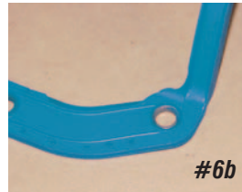
Photo #6a & 6b: Here is the answer to this long-time problem; a one-piece oil pan gasket! The new one-piece oil pan gasket is preformed silicone with steel ring inserts at each bolt hole. The steel rings allow the oil pan bolt to crush the gasket perfectly for sealing, but not too tight to push the gasket out.
